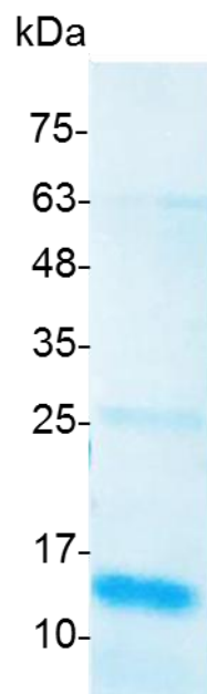
SDS-PAGE analysis of recombinant human BMP-3
