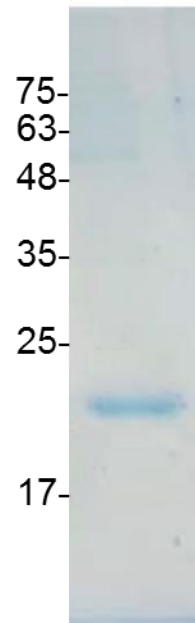
SDS-PAGE analysis of recombinant mouse IL-33
